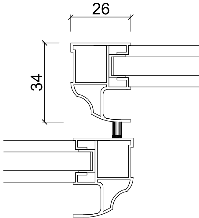
Slide Wing
